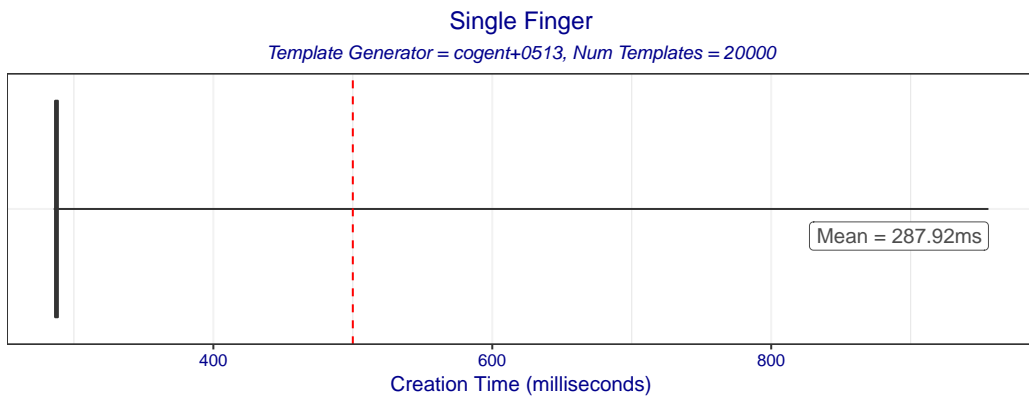
Figure 2: Boxplot of template creation times for template generator cogent+0513. The box edges mark the 10th and 90th percentiles while the whiskers mark the maximum and minimum creation times.
