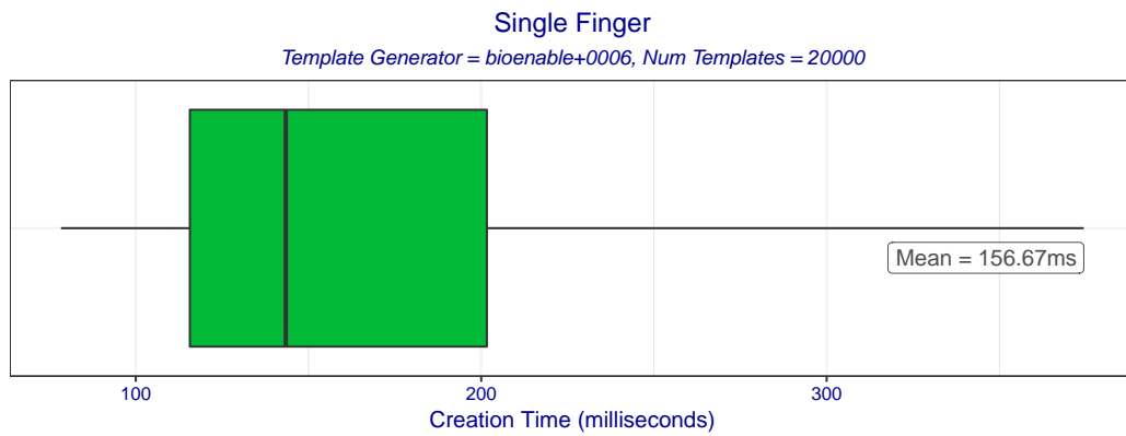
Figure 2: Boxplot of template creation times for template generator bioenable+0006. The box edges mark the 10th and 90th percentiles while the whiskers mark the maximum and minimum creation times.
