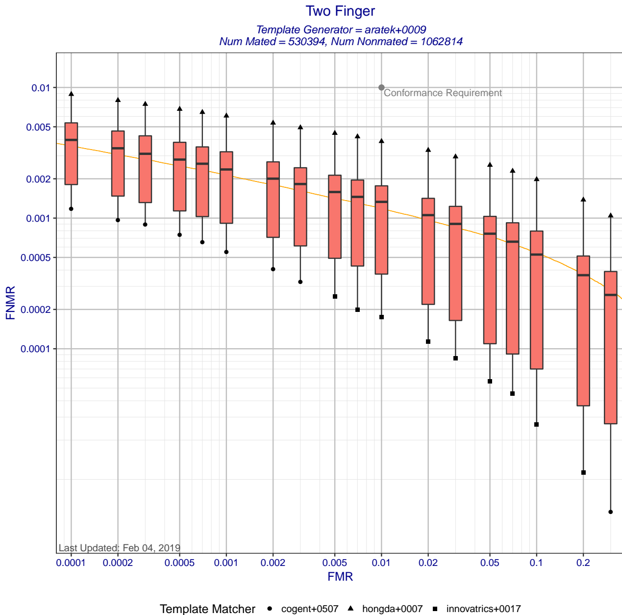
Figure 6: Two Finger DET statistics for template generator aratek+0009. Each box shows the distribution of FNMRs at a fixed FMR across different matchers. The whisker ends show the minimum and maximum FNMRs. The orange DET curve shows pooled performance when all matchers use templates created by aratek+0009. Score-level fusion is achieved by averaging the scores for left and right index fingers.
