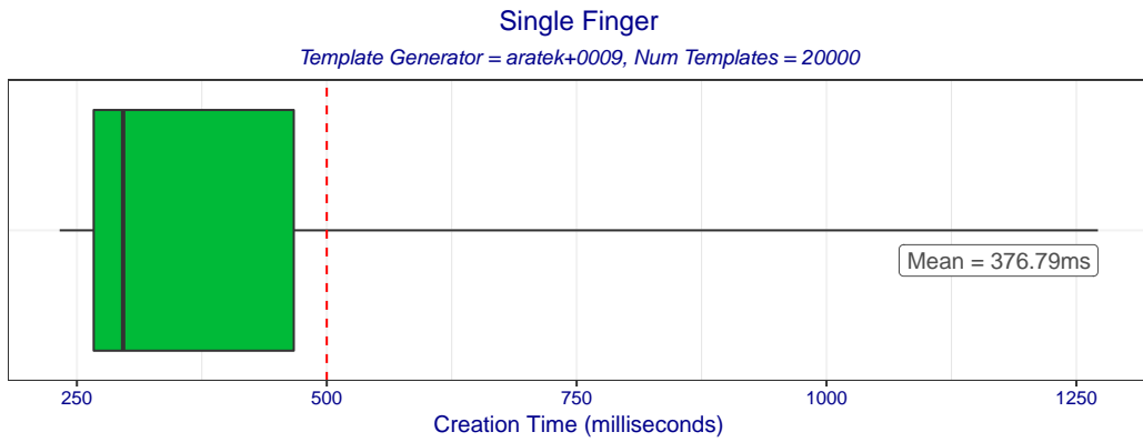
Figure 8: Boxplot of template creation times for template generator aratek+0009. The box edges mark the 10th and 90th percentiles while the whiskers mark the maximum and minimum creation times.
