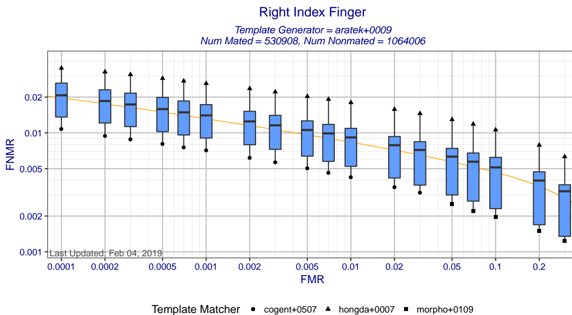
Figure 3: Right Index Finger DET statistics for template generator aratek+0009. Each box shows the distribution of FNMRs at a fixed FMR across different matchers. The whisker ends show the minimum and maximum FNMRs. The orange DET curve shows pooled performance when all matchers use templates created by aratek+0009.
