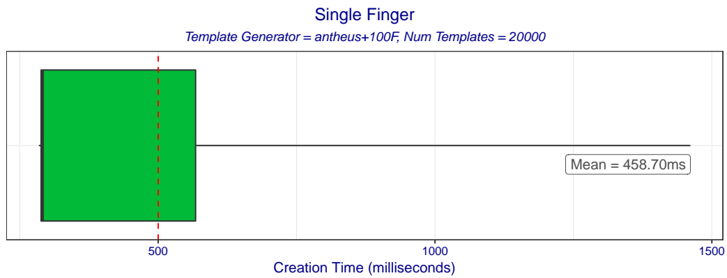
Figure 2: Boxplot of template creation times for template generator antheus+100F. The box edges mark the 10th and 90th percentiles while the whiskers mark the maximum and minimum creation times.
