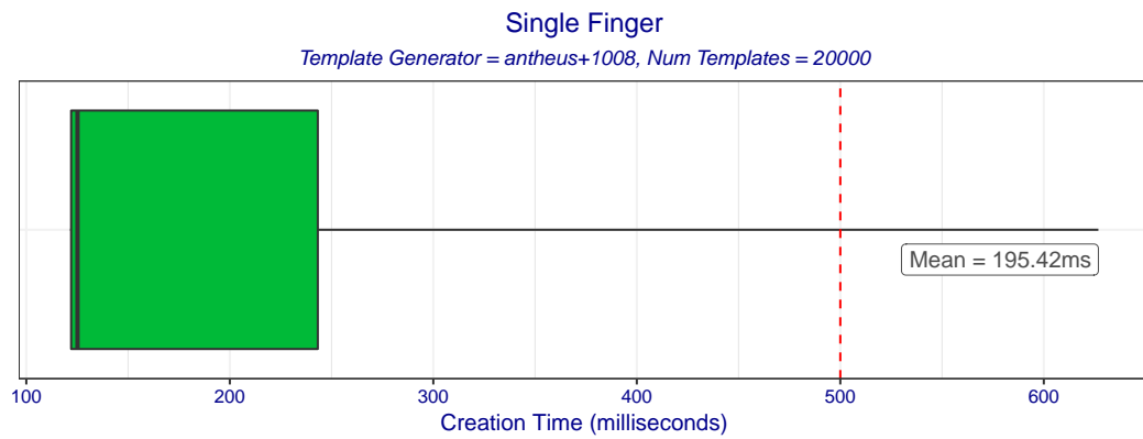
Figure 2: Boxplot of template creation times for template generator antheus+1008. The box edges mark the 10th and 90th percentiles while the whiskers mark the maximum and minimum creation times.
