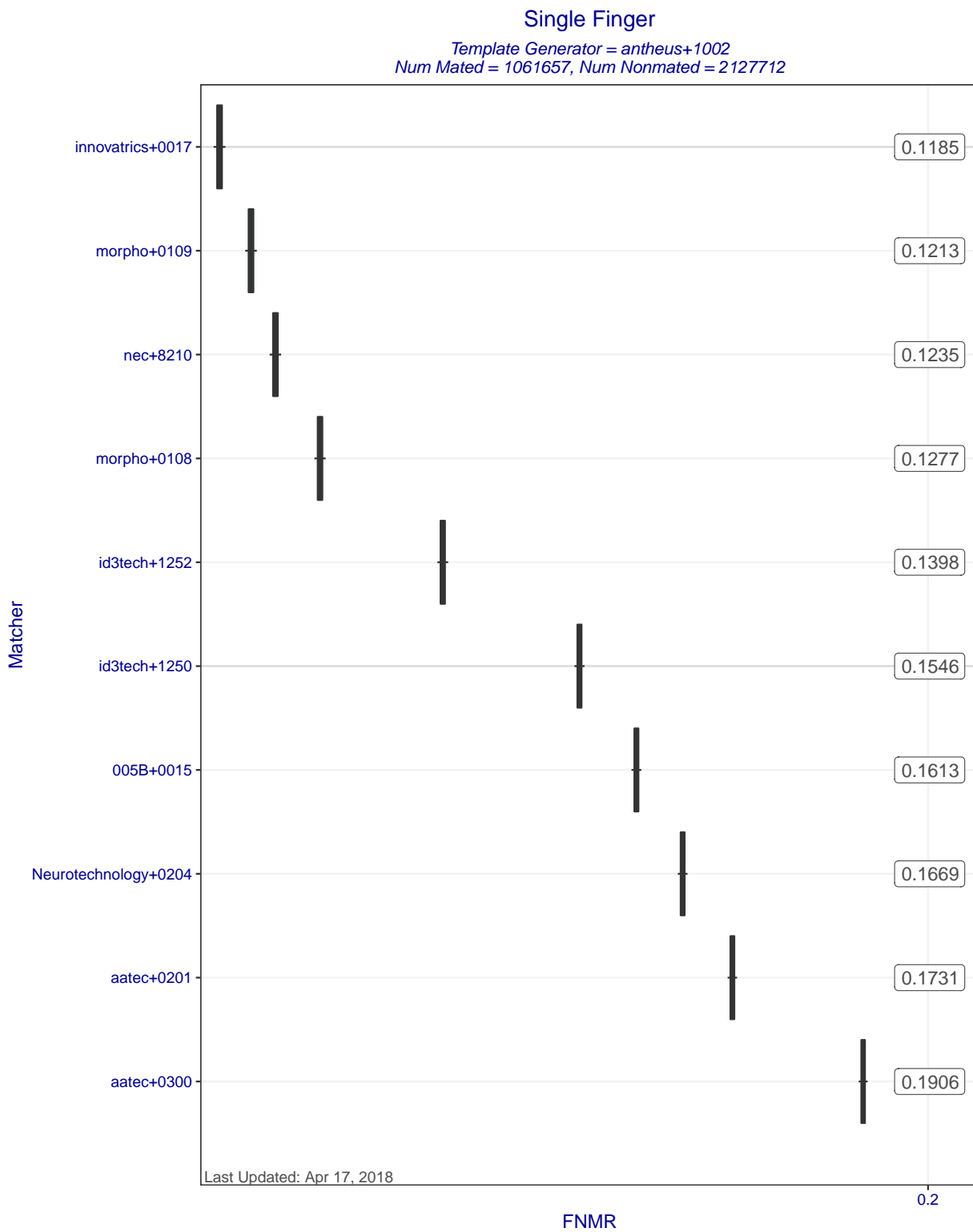
Figure 5: Single Finger FNMRs at FMR=0.0001 when MINEX III compliant matchers compare templates created by template generator antheus+1002. Each box represents uncertainty about the true FNMR. The box edges mark the 50% confidence intervals while the whiskers mark the 90% confidence intervals. The numbers on the right show the actual computed FNMRs.
