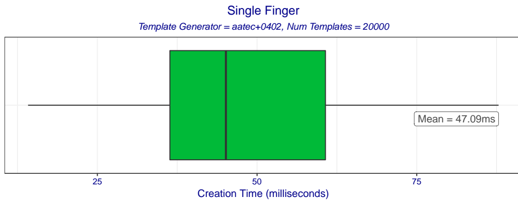
Figure 2: Boxplot of template creation times for template generator aatec+0402. The box edges mark the 10th and 90th percentiles while the whiskers mark the maximum and minimum creation times.
