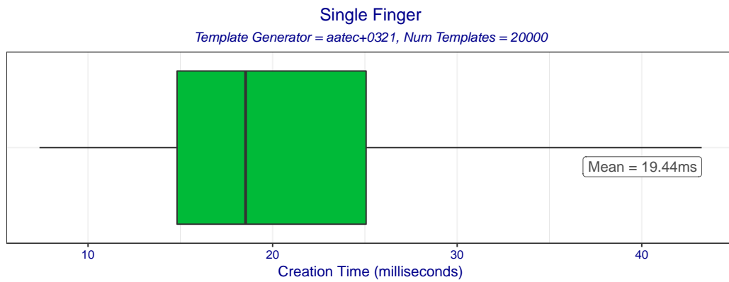
Figure 2: Boxplot of template creation times for template generator aatec+0321. The box edges mark the 10th and 90th percentiles while the whiskers mark the maximum and minimum creation times.
