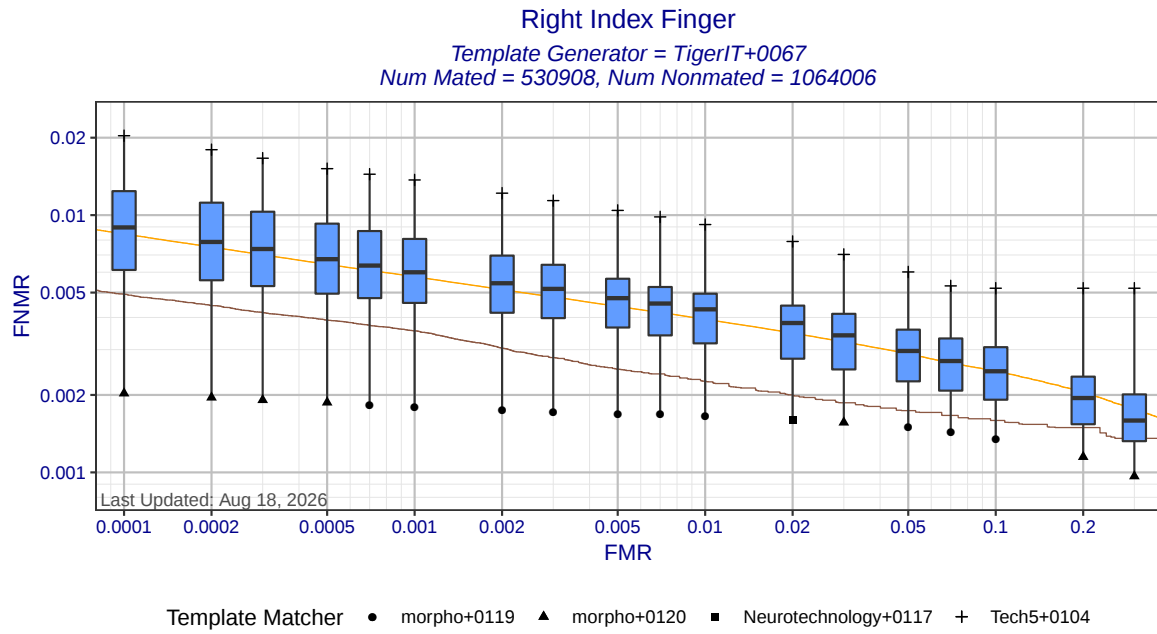
Figure 3: Right Index Finger DET statistics for template generator TigerIT+0067. Each box shows the distribution of FNMRs at a fixed FMR across different matchers. The whisker ends show the minimum and maximum FNMRs. The brown curve shows the DET curve when the matcher and template generators were submitted by the same participant. The orange DET curve shows pooled performance when all matchers use templates created by TigerIT+0067.
