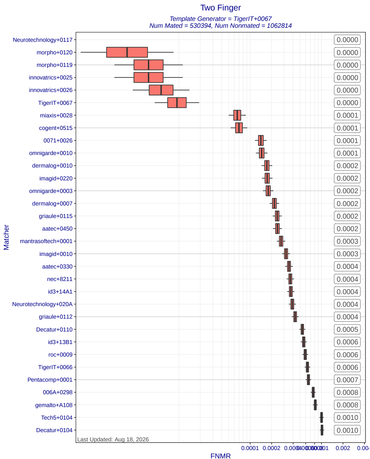
Figure 7: Two Finger FNMR at FMR=0.01 when different matchers compare templates created by template generator TigerIT+0067. Each box represents uncertainty about the true FNMR. The box edges mark the 50% confidence intervals while the whiskers mark the 90% confidence intervals. The numbers on the right show the actual computed FNMRs. Score-level fusion is achieved by averaging the scores for left and right index fingers.
