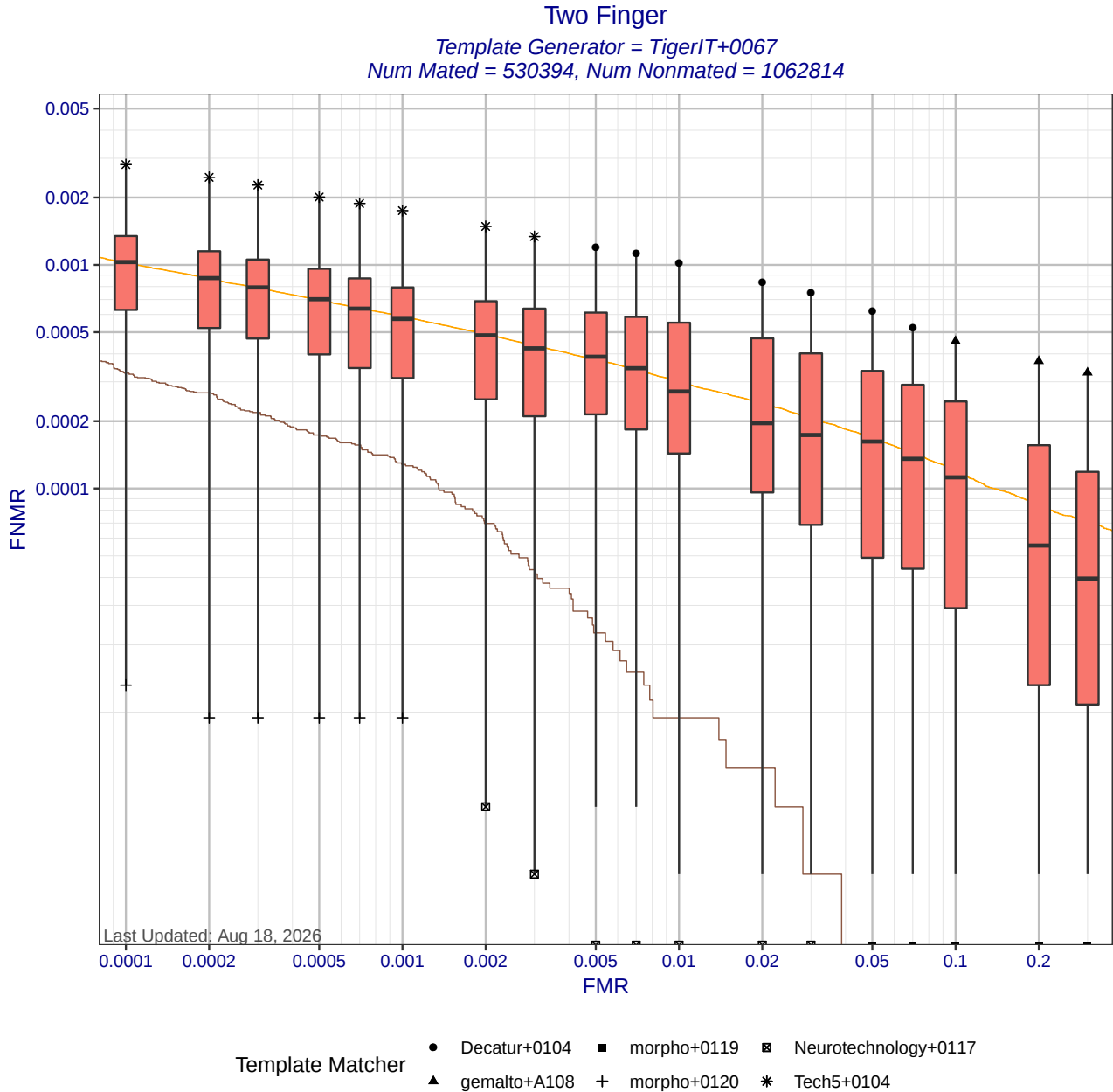
Figure 6: Two Finger DET statistics for template generator TigerIT+0067. Each box shows the distribution of FNMRs at a fixed FMR across different matchers. The whisker ends show the minimum and maximum FNMRs. The brown curve shows the DET curve when the matcher and template generators were submitted by the same participant. The orange DET curve shows pooled performance when all matchers use templates created by TigerIT+0067. Score-level fusion is achieved by averaging the scores for left and right index fingers.
