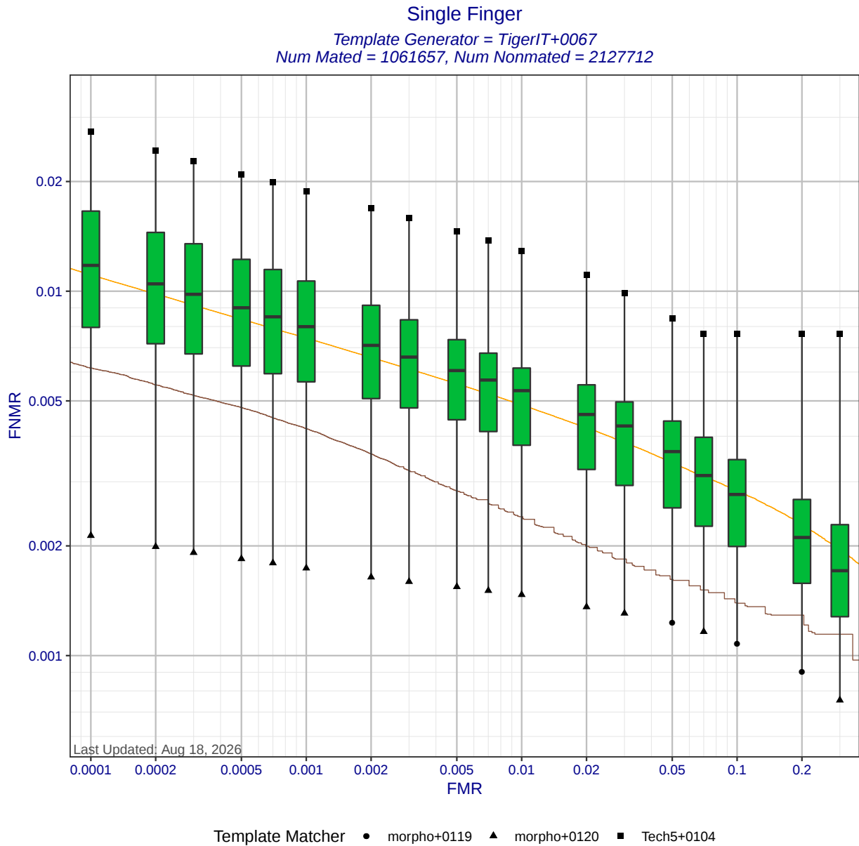
Figure 2: Single finger DET statistics for template generator TigerIT+0067. Each box shows the distribution of FNMRs at a fixed FMR across different matchers. The whisker ends show the minimum and maximum FNMRs. The brown curve shows the DET curve when the matcher and template generators were submitted by the same participant. The orange DET curve shows pooled performance when all matchers compare templates created by TigerIT+0067.
