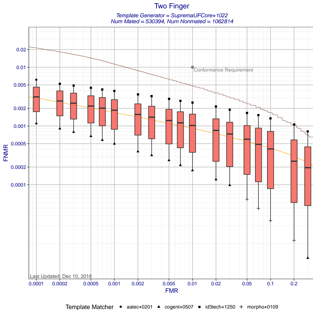
Figure 6: Two Finger DET statistics for template generator SupremaUFCore+1022. Each box shows the distribution of FNMRs at a fixed FMR across different matchers. The whisker ends show the minimum and maximum FNMRs. The brown curve shows the DET curve when the matcher and template generators were submitted by the same participant. The orange DET curve shows pooled performance when all matchers use templates created by SupremaUFCore+1022. Score-level fusion is achieved by averaging the scores for left and right index fingers.
