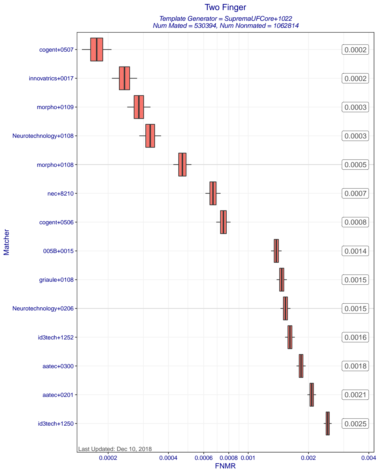
Figure 7: Two Finger FNMR at FMR=0.01 when different matchers compare templates created by template generator SupremaUFCore+1022. Each box represents uncertainty about the true FNMR. The box edges mark the 50% confidence intervals while the whiskers mark the 90% confidence intervals. The numbers on the right show the actual computed FNMRs. Score-level fusion is achieved by averaging the scores for left and right index fingers.
