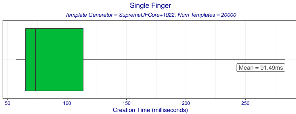
Figure 8: Boxplot of template creation times for template generator SupremaUFCore+1022. The box edges mark the 10th and 90th percentiles while the whiskers mark the maximum and minimum creation times.
