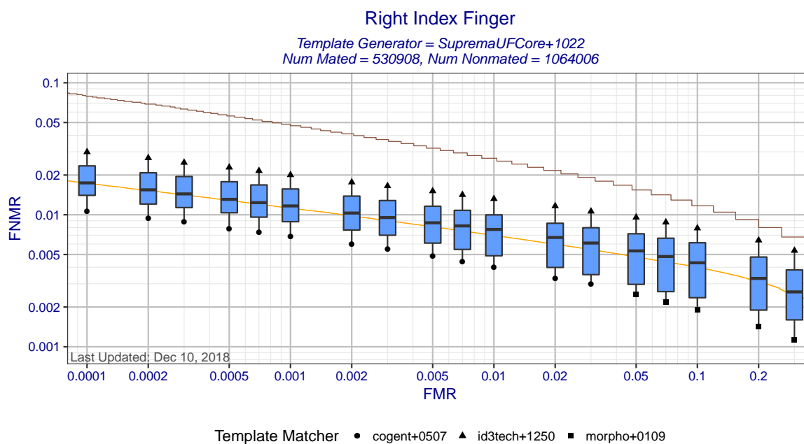
Figure 3: Right Index Finger DET statistics for template generator SupremaUFCore+1022. Each box shows the distribution of FNMRs at a fixed FMR across different matchers. The whisker ends show the minimum and maximum FNMRs. The brown curve shows the DET curve when the matcher and template generators were submitted by the same participant. The orange DET curve shows pooled performance when all matchers use templates created by SupremaUFCore+1022.
