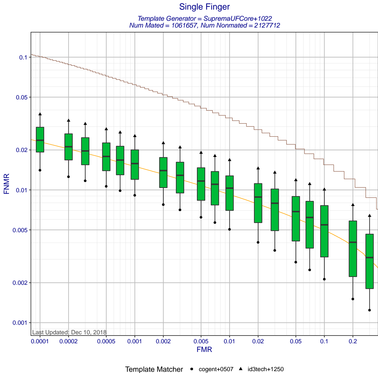
Figure 2: Single finger DET statistics for template generator SupremaUFCore+1022. Each box shows the distribution of FNMRs at a fixed FMR across different matchers. The whisker ends show the minimum and maximum FNMRs. The brown curve shows the DET curve when the matcher and template generators were submitted by the same participant. The orange DET curve shows pooled performance when all matchers compare templates created by SupremaUFCore+1022.
