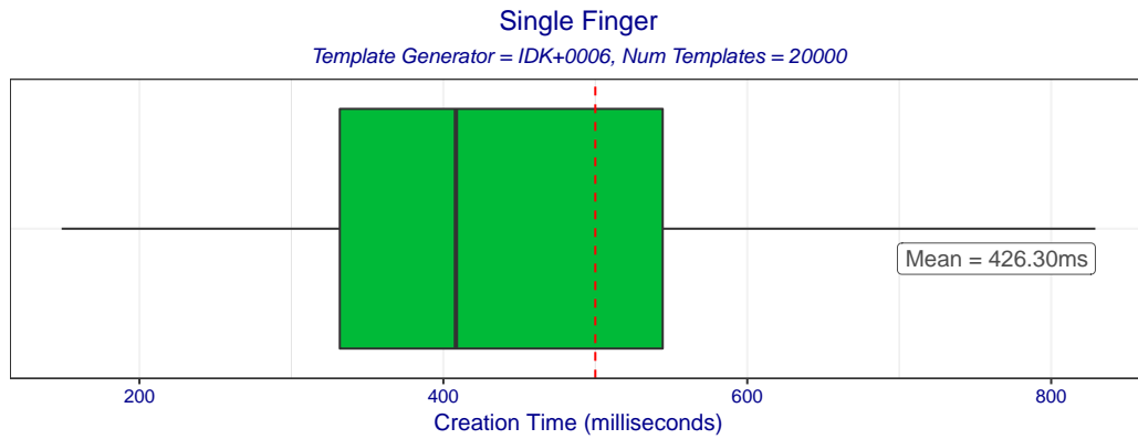
Figure 2: Boxplot of template creation times for template generator IDK+0006. The box edges mark the 10th and 90th percentiles while the whiskers mark the maximum and minimum creation times.
