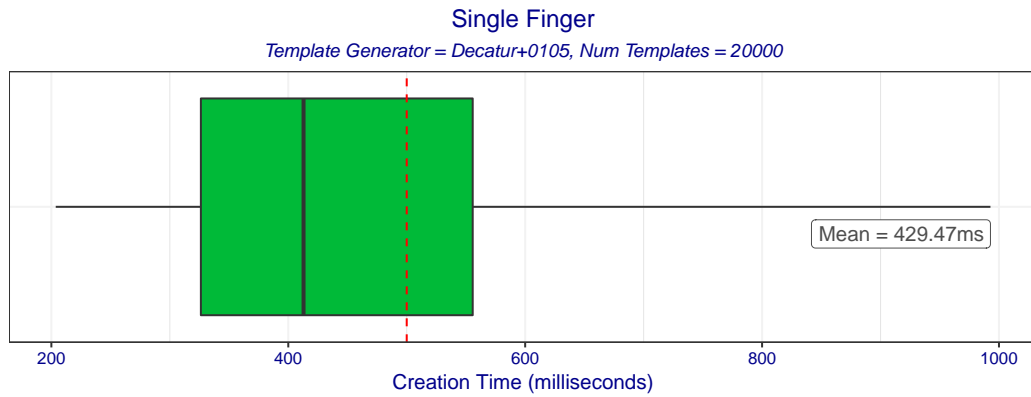
Figure 2: Boxplot of template creation times for template generator Decatur+0105. The box edges mark the 10th and 90th percentiles while the whiskers mark the maximum and minimum creation times.
