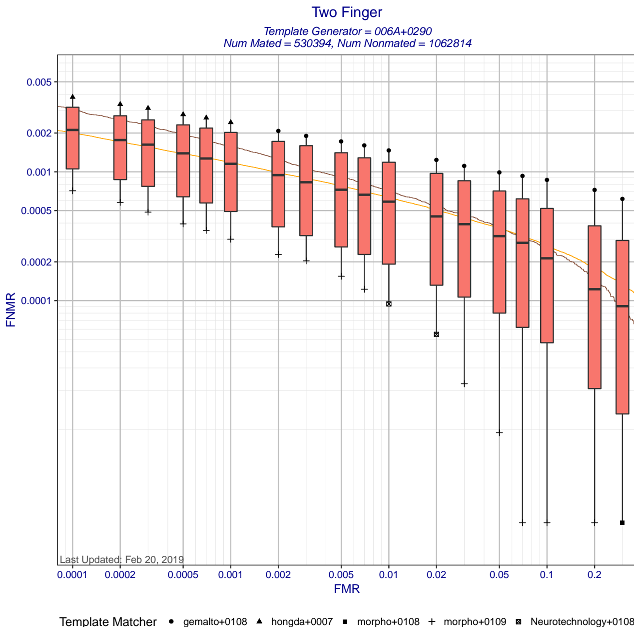
Figure 6: Two Finger DET statistics for template generator 006A+0290. Each box shows the distribution of FNMRs at a fixed FMR across different matchers. The whisker ends show the minimum and maximum FNMRs. The brown curve shows the DET curve when the matcher and template generators were submitted by the same participant. The orange DET curve shows pooled performance when all matchers use templates created by 006A+0290. Score-level fusion is achieved by averaging the scores for left and right index fingers.
