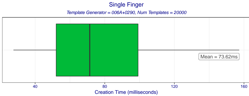
Figure 8: Boxplot of template creation times for template generator 006A+0290. The box edges mark the 10th and 90th percentiles while the whiskers mark the maximum and minimum creation times.
