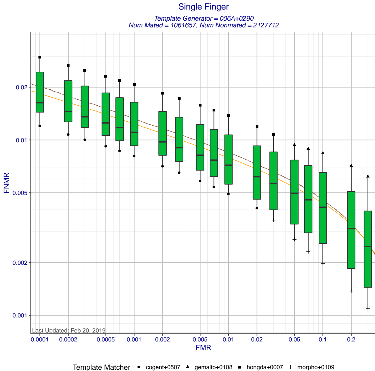
Figure 2: Single finger DET statistics for template generator 006A+0290. Each box shows the distribution of FNMRs at a fixed FMR across different matchers. The whisker ends show the minimum and maximum FNMRs. The brown curve shows the DET curve when the matcher and template generators were submitted by the same participant. The orange DET curve shows pooled performance when all matchers compare templates created by 006A+0290.
