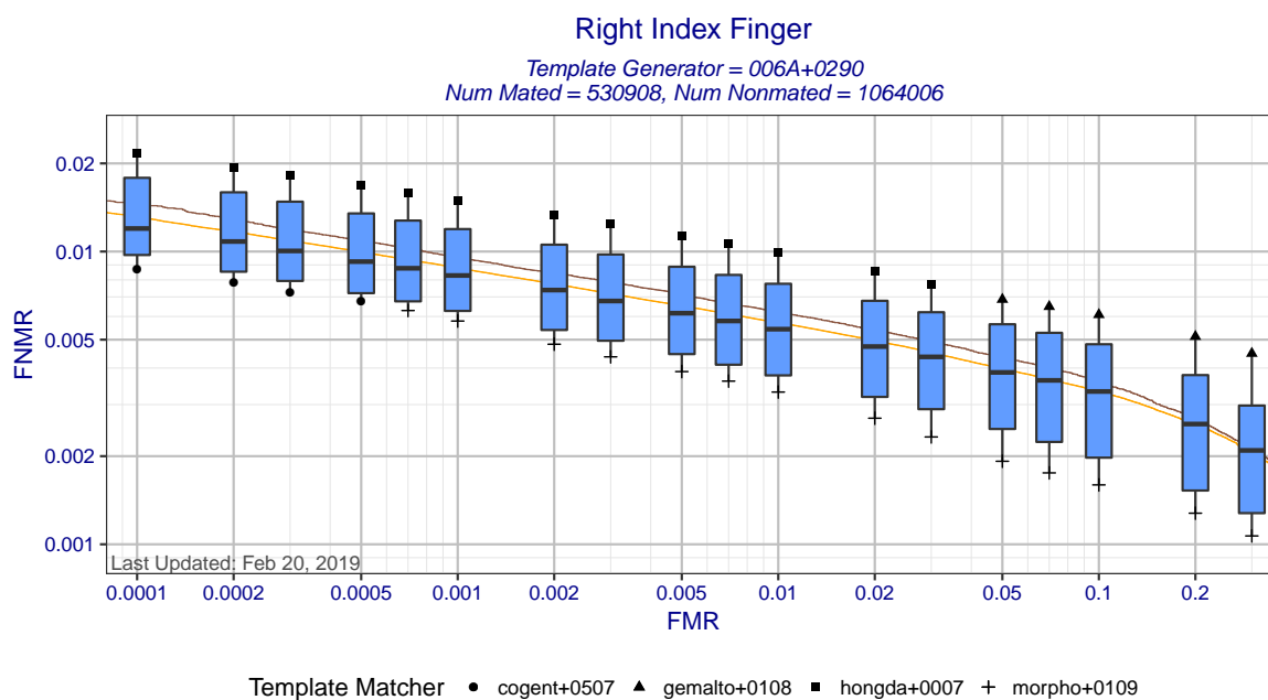
Figure 3: Right Index Finger DET statistics for template generator 006A+0290. Each box shows the distribution of FNMRs at a fixed FMR across different matchers. The whisker ends show the minimum and maximum FNMRs. The brown curve shows the DET curve when the matcher and template generators were submitted by the same participant. The orange DET curve shows pooled performance when all matchers use templates created by 006A+0290.
