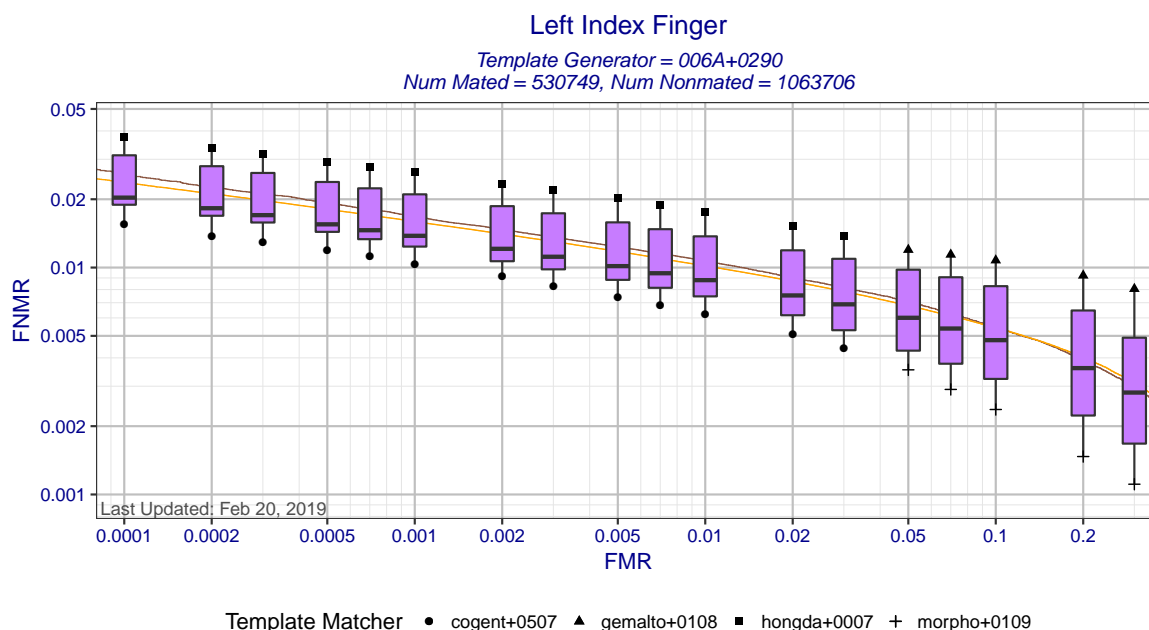
Figure 4: Left Index Finger DET statistics for template generator 006A+0290. Each box shows the distribution of FNMRs at a fixed FMR across different template generators. The brown curve shows the DET curve when the matcher and template generators were submitted by the same participant. The orange DET curve shows pooled performance when all matchers use templates created by 006A+0290.
