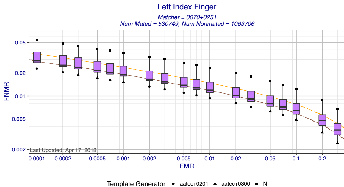
Figure 4: Left index finger DET statistics for matcher 0070+0251. Each box shows the distribution of FNMRs at a fixed FMR across all MINEX III compliant template generators. The ends of whiskers show the minimum and maximum FNMRs. The orange DET curve shows pooled performance against all template generators.
