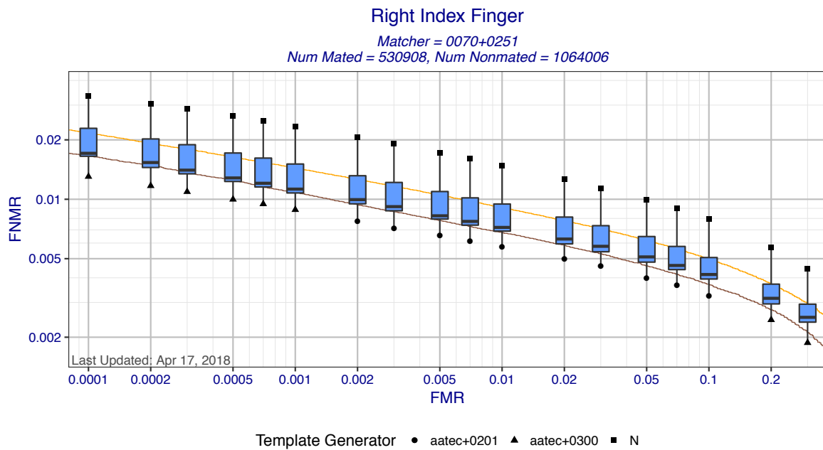
Figure 3: Right index finger DET statistics for matcher 0070+0251. Each box shows the distribution of FNMR at a fixed FMR across all MINEX III compliant template generators. The ends of the whiskers show the minimum and maximum FNMRs. The orange DET curve shows pooled performance against all template generators.
