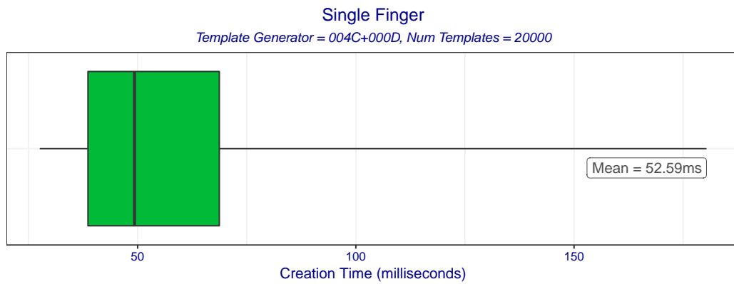
Figure 2: Boxplot of template creation times for template generator 004C+000D. The box edges mark the 10th and 90th percentiles while the whiskers mark the maximum and minimum creation times.
