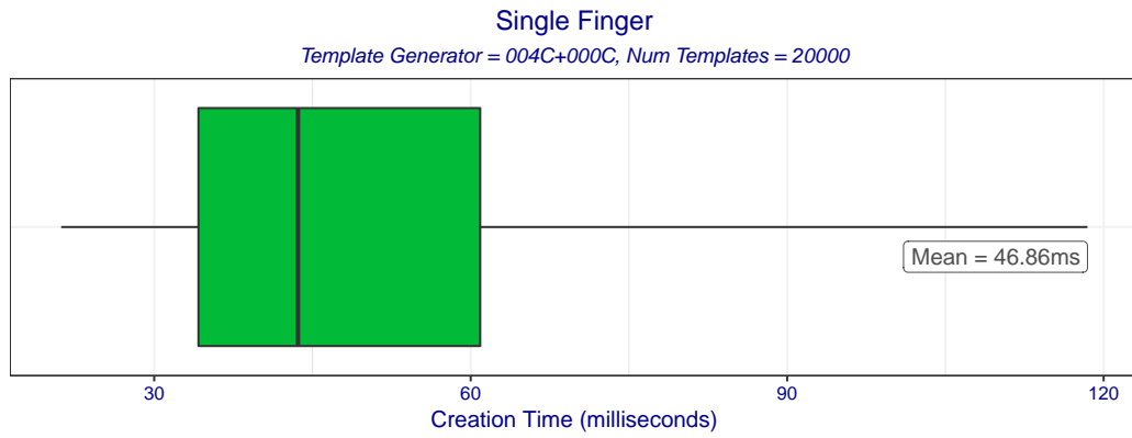
Figure 2: Boxplot of template creation times for template generator 004C+000C. The box edges mark the 10th and 90th percentiles while the whiskers mark the maximum and minimum creation times.
