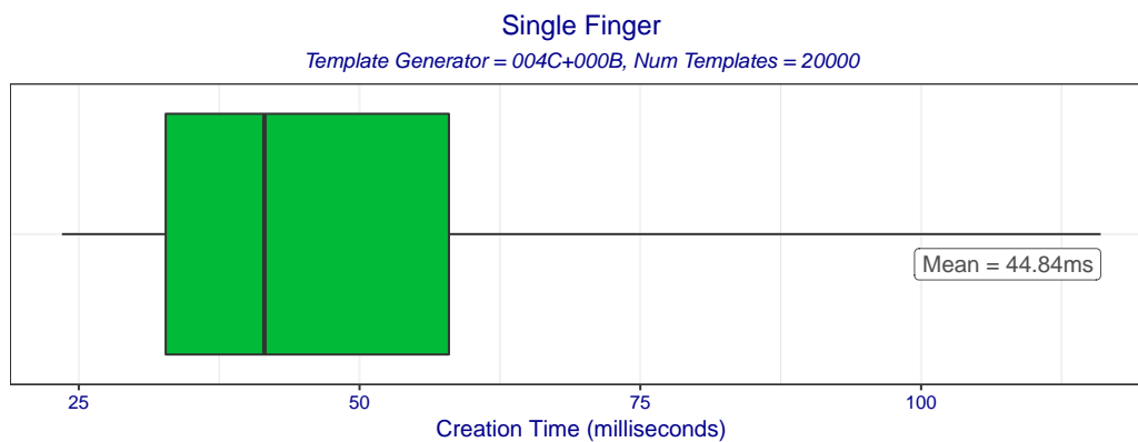
Figure 2: Boxplot of template creation times for template generator 004C+000B. The box edges mark the 10th and 90th percentiles while the whiskers mark the maximum and minimum creation times.
