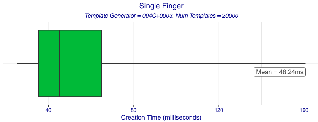
Figure 2: Boxplot of template creation times for template generator 004C+0003. The box edges mark the 10th and 90th percentiles while the whiskers mark the maximum and minimum creation times.
