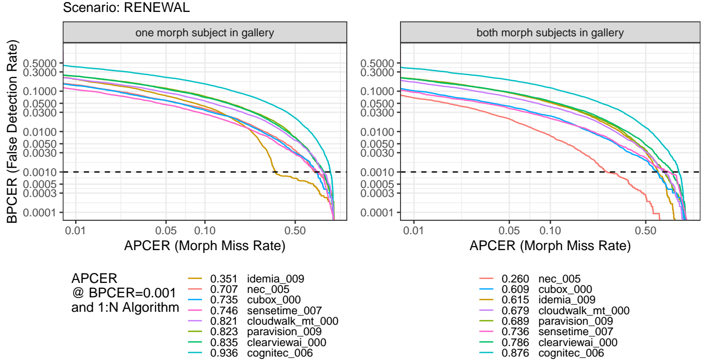
Figure 8: Accuracy of morph classifiers trained on different 1:N algorithm rank 1 + 2 scores for morphed searches (one or both subjects in gallery) and mated bona fide searches against a consolidated gallery.
