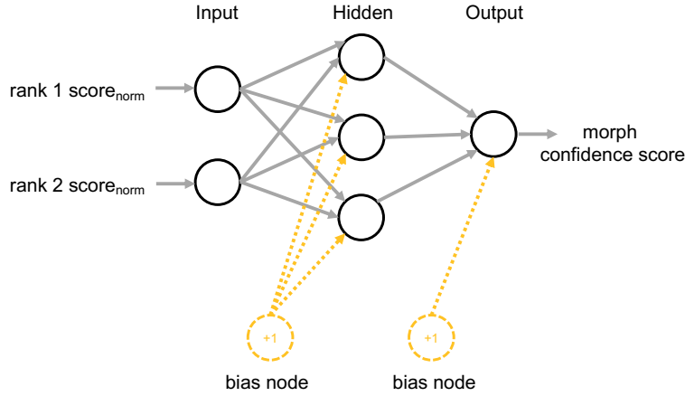
Figure 7: Neural network architecture for training a morph classifier with 1:N algorithm rank 1 and 2 scores. A sigmoid function is used in the the hidden and output layers.
