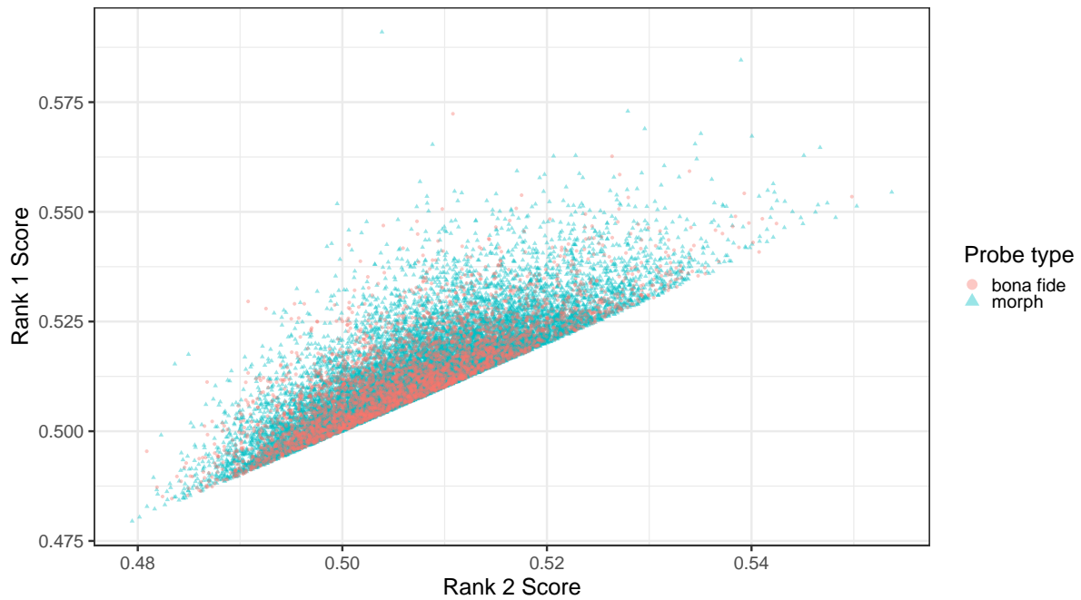
Figure 15: This plot combines the rank 1 and 2 scores from the bona fide and morph search scenarios against an consolidated gallery from Figure 14.
