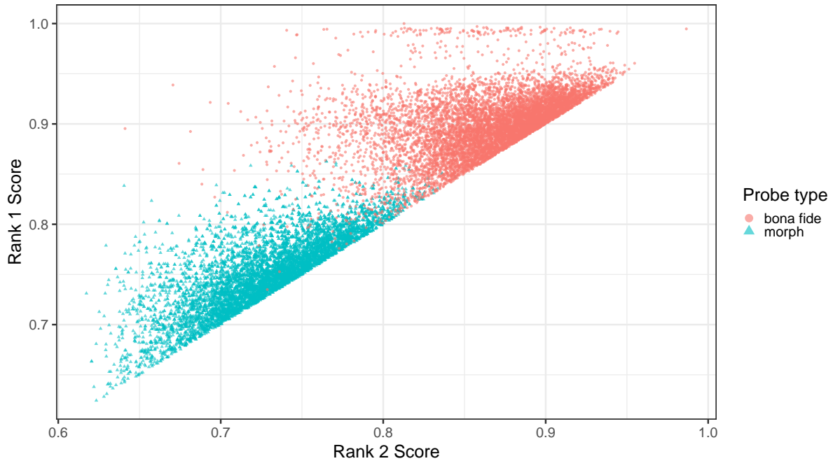
Figure 11: This plot combines the rank 1 and 2 scores from the various bona fide and morph search scenarios against an unconsolidated gallery from Figure 10.
