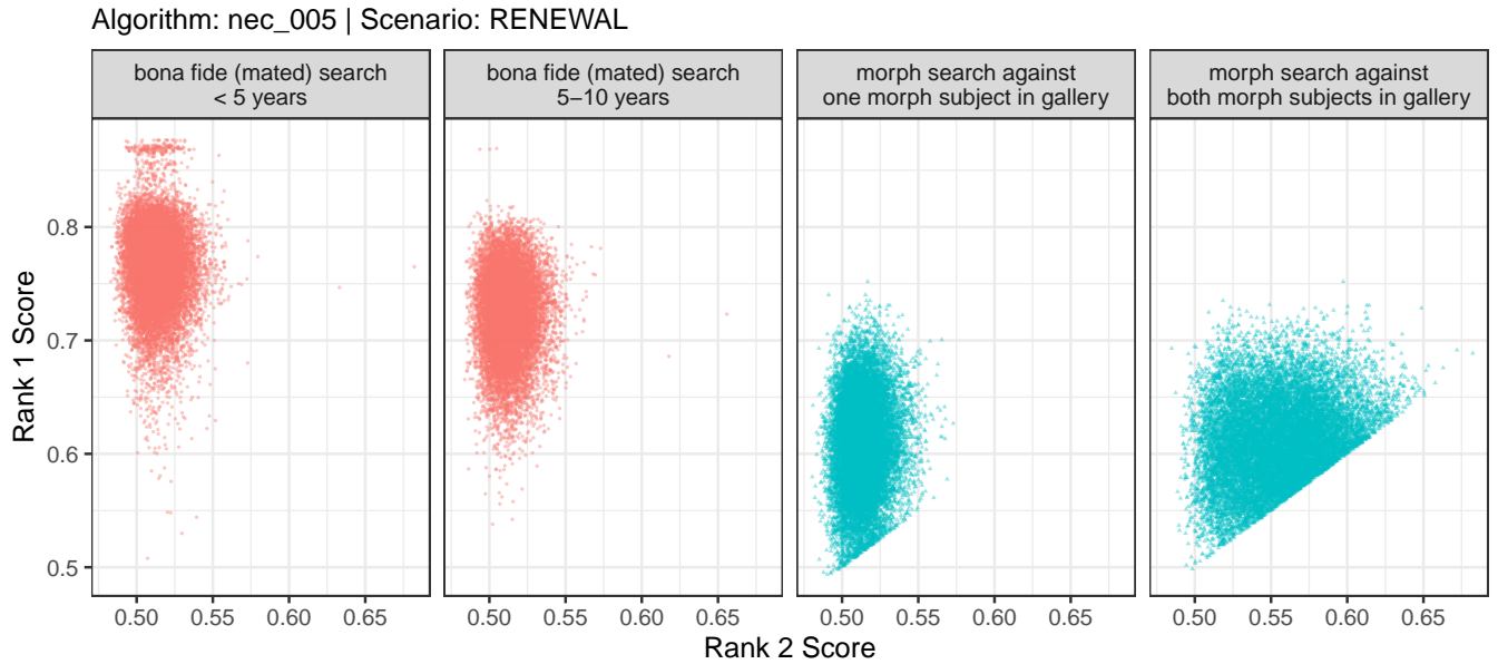
Figure 5: The position of each point in the scatter plot represents the native rank 1 and 2 similarity scores for bona fide or morph probes searched against a consolidated gallery that contains a prior photo of the subject(s). For bona fides, the probes are broken out by the age difference between the probe and the gallery image (< 5 years and 5 - 10 years). For morphs, scores are shown for galleries that include either one subject or both subjects that went into the morph. All galleries contain 1.6 million unique people.
