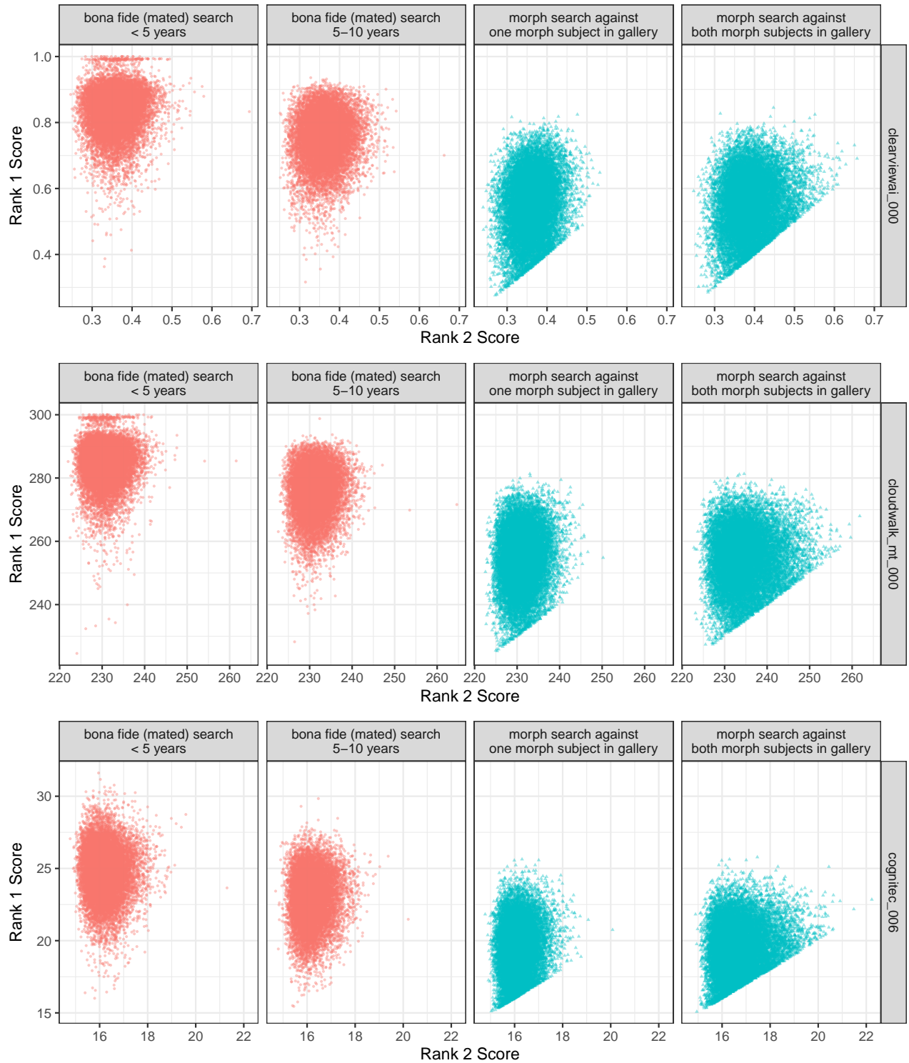
Figure 17: The scatter plots show native 1:N algorithm rank 1 and 2 similarity scores for bona fide or morph probes searched against a consolidated gallery that contains a prior photo of the subject(s). For bona fides, scores are broken out by the time elapsed (< 5 years or between 5 - 10 years) between the probe and gallery photo. For morphs, scores are shown for galleries that include either one subject or both subjects that went into the morph. All galleries contain 1.6 million unique people.
