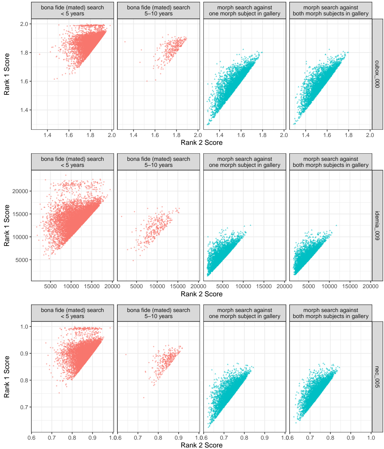
Figure 21: The scatter plots show native 1:N algorithm rank 1 and 2 similarity scores for bona fide or morph probes searched against an unconsolidated gallery that contains multiple (two or more) prior photos of the subject(s). For bona fides, scores are broken out by the time elapsed (< 5 years or between 5 - 10 years) between the probe and gallery photos. For morphs, scores are shown for galleries that include either one subject or both subjects that went into the morph. All galleries contain 1.6 million unique people.
