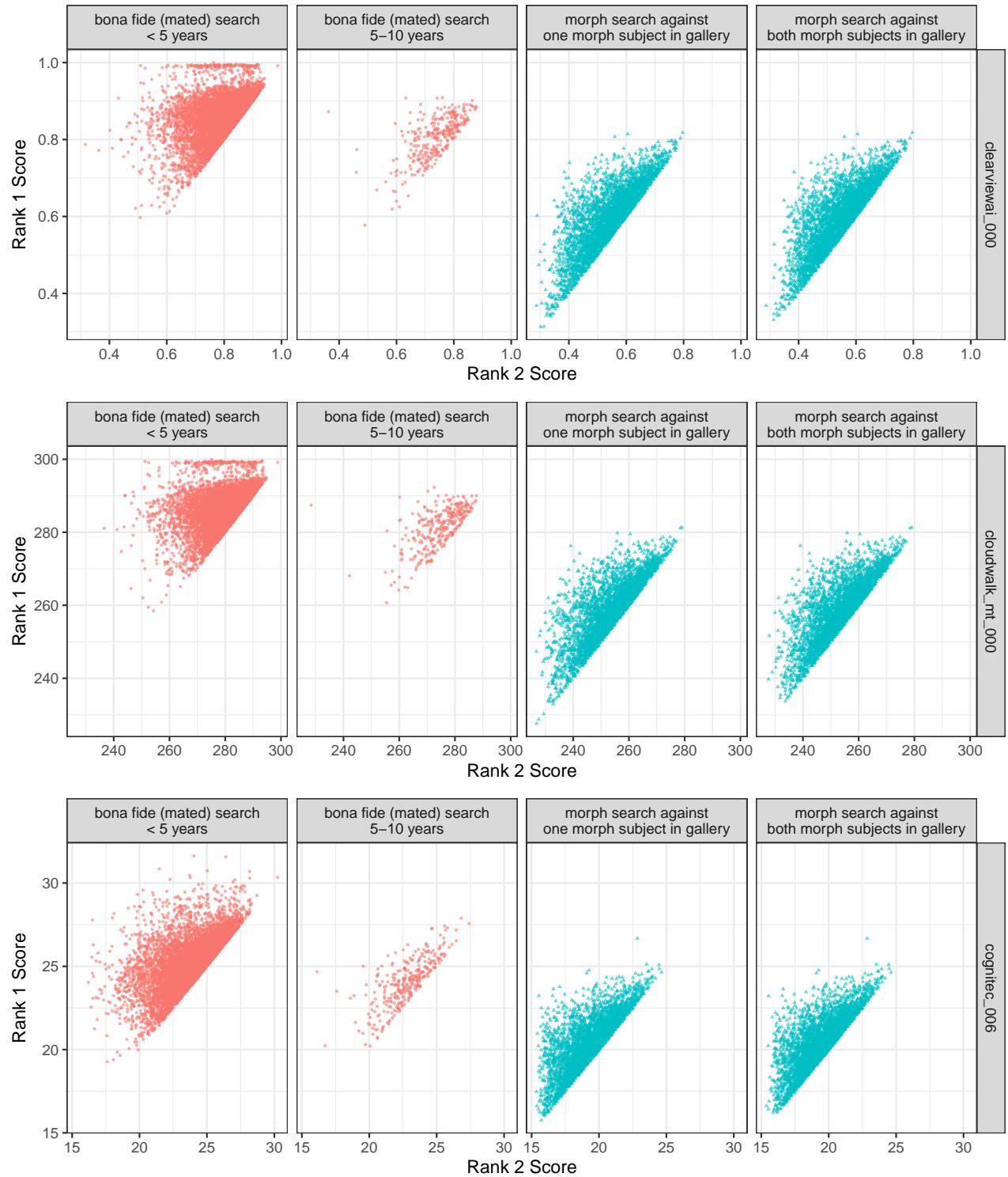
Figure 20: The scatter plots show native 1:N algorithm rank 1 and 2 similarity scores for bona fide or morph probes searched against an unconsolidated gallery that contains multiple (two or more) prior photos of the subject(s). For bona fides, scores are broken out by the time elapsed (< 5 years or between 5 - 10 years) between the probe and gallery photos. For morphs, scores are shown for galleries that include either one subject or both subjects that went into the morph. All galleries contain 1.6 million unique people.
