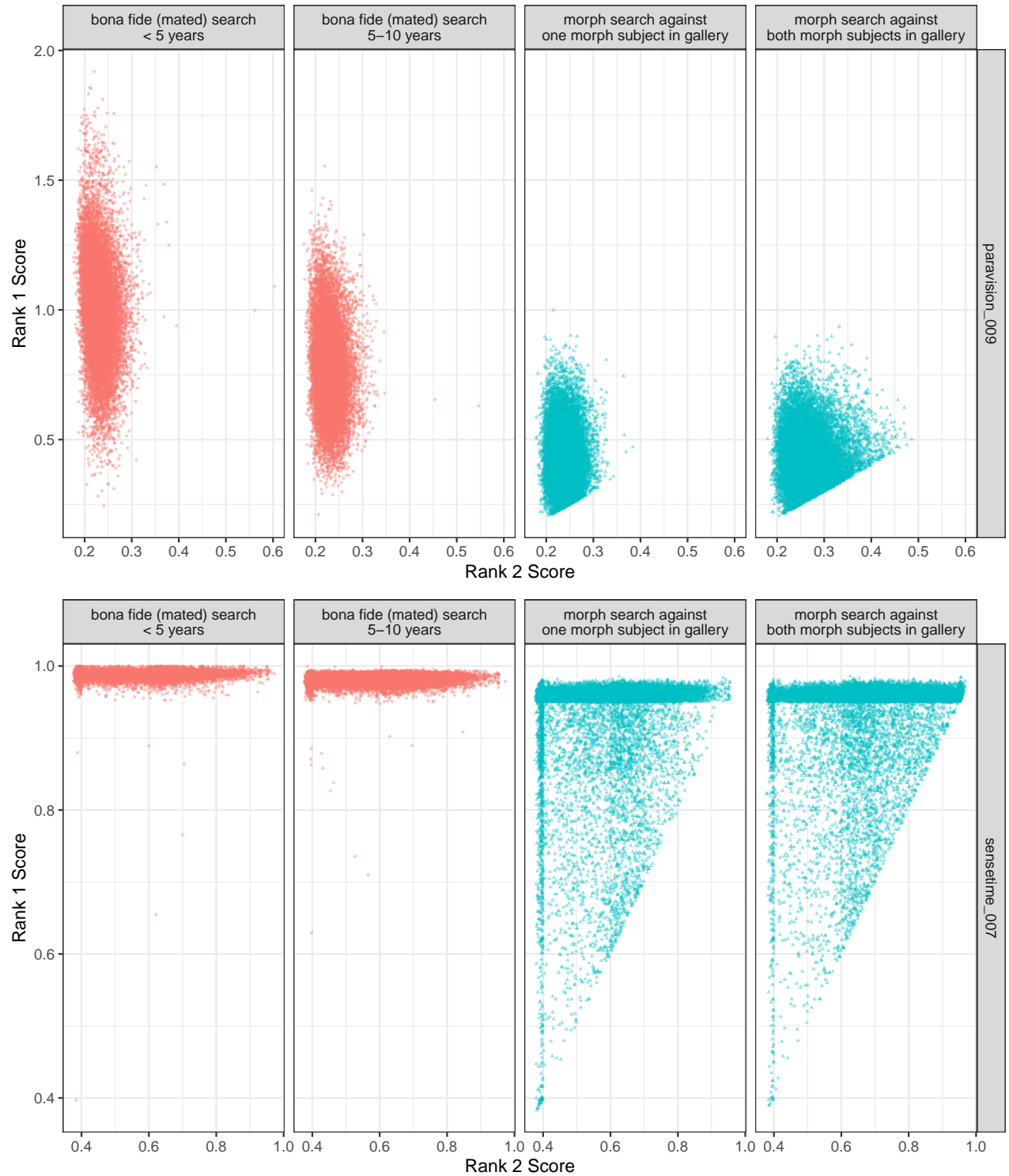
Figure 19: The scatter plots show native 1:N algorithm rank 1 and 2 similarity scores for bona fide or morph probes searched against a consolidated gallery that contains a prior photo of the subject(s). For bona fides, scores are broken out by the time elapsed (< 5 years or between 5 - 10 years) between the probe and gallery photo. For morphs, scores are shown for galleries that include either one subject or both subjects that went into the morph. All galleries contain 1.6 million unique people.
