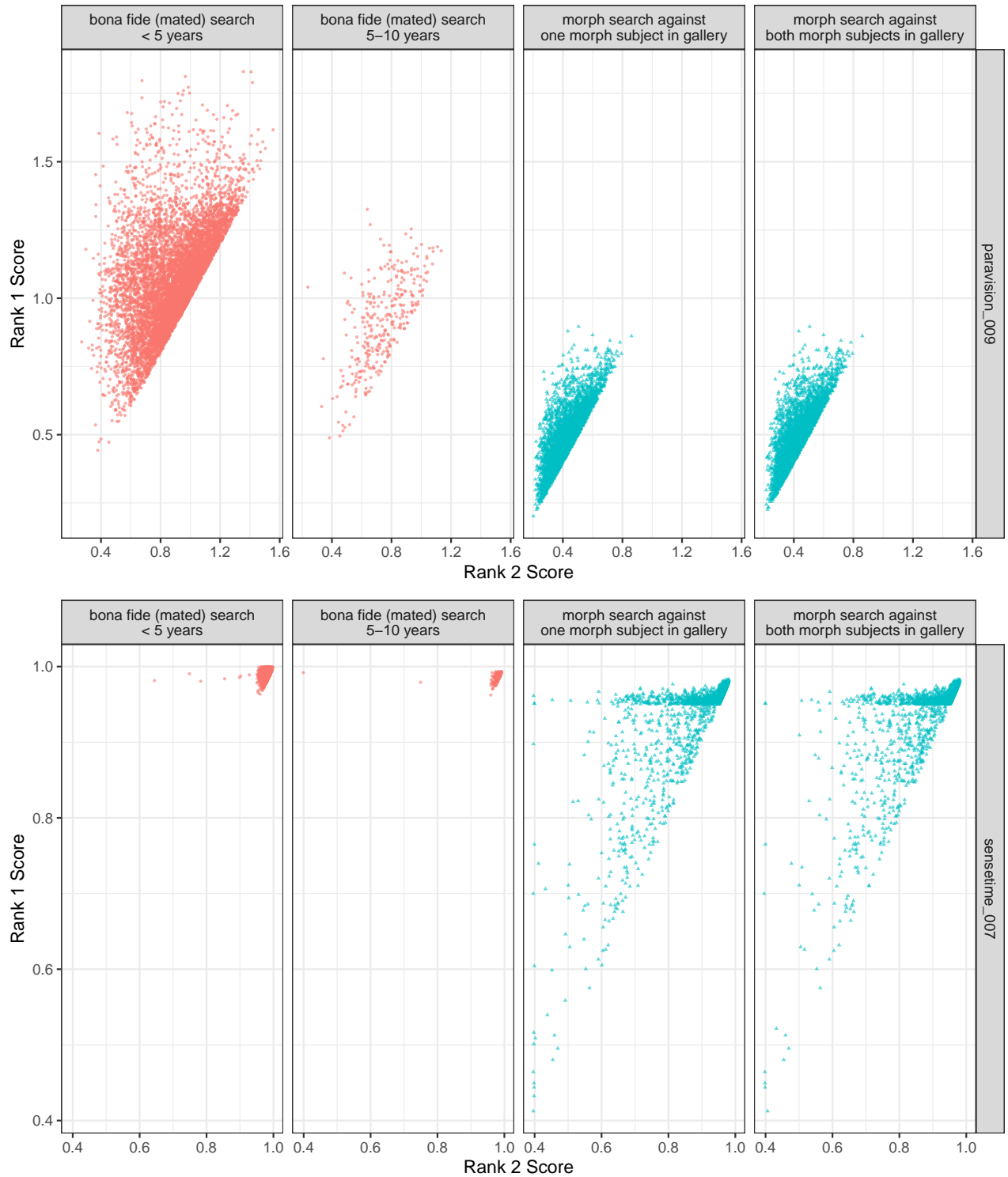
Figure 22: The scatter plots show native 1:N algorithm rank 1 and 2 similarity scores for bona fide or morph probes searched against an unconsolidated gallery that contains multiple (two or more) prior photos of the subject(s). For bona fides, scores are broken out by the time elapsed (< 5 years or between 5 - 10 years) between the probe and gallery photos. For morphs, scores are shown for galleries that include either one subject or both subjects that went into the morph. All galleries contain 1.6 million unique people.
