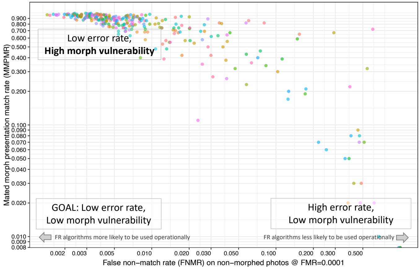
Figure 1: This graph plots face recognition algorithm vulnerability on morphs against general algorithm accuracy on non-morphed photos. Each point represents a face recognition algorithm recently submitted to the NIST FRVT 1:1 activity. The y-axis plots MMPMR, which is the fraction of morphs where both subjects incorrectly match to the morph. The x-axis plots FNMR or miss rate on regular photos, which provides an indication of general algorithm accuracy. Both MMPMR and FNMR are calculated with thresholds set to where the false match rate (FMR) is 0.0001. The morphs were generated with two people with equal contribution from each subject.
