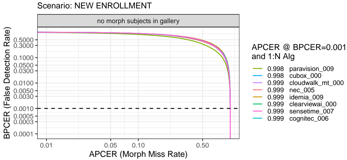
Figure 16: Accuracy of morph classifiers trained on different 1:N algorithm rank 1 + 2 scores for morphed or bona fide searches against a consolidated gallery when no prior photos of the subjects exist in the gallery.
