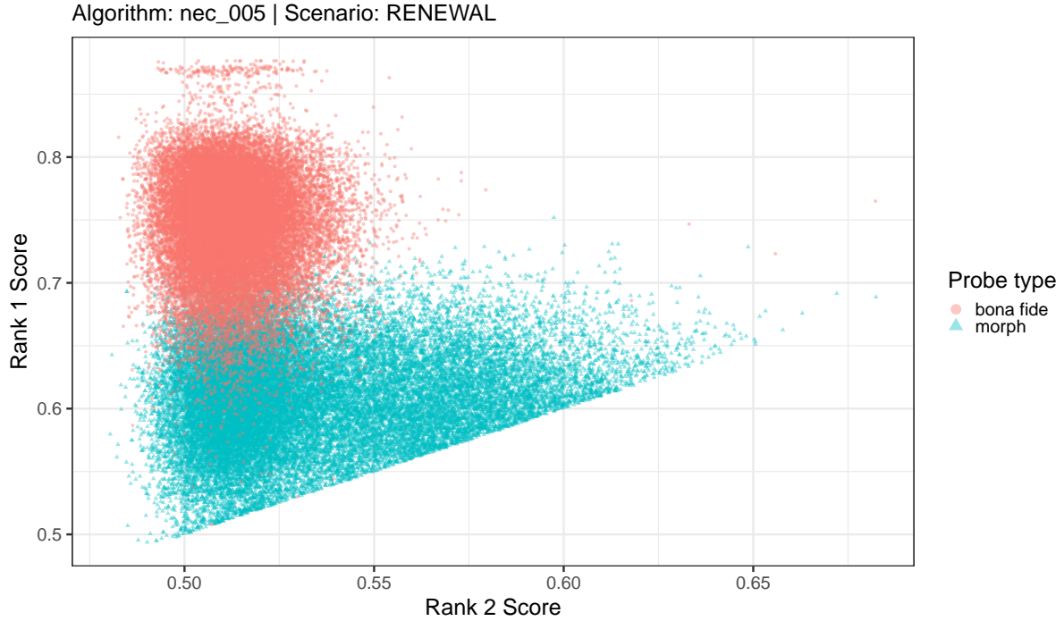
Figure 6: This plot combines the rank 1 and 2 scores from the various bona fide and morph search scenarios against a consolidated gallery from Figure 5.
