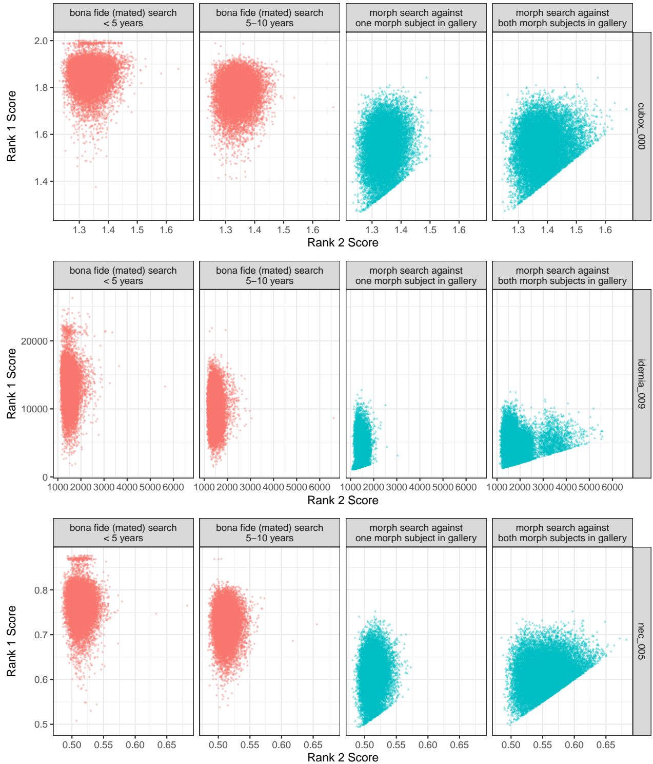
Figure 18: The scatter plots show native 1:N algorithm rank 1 and 2 similarity scores for bona fide or morph probes searched against a consolidated gallery that contains a prior photo of the subject(s). For bona fides, scores are broken out by the time elapsed (< 5 years or between 5 - 10 years) between the probe and gallery photo. For morphs, scores are shown for galleries that include either one subject or both subjects that went into the morph. All galleries contain 1.6 million unique people.
