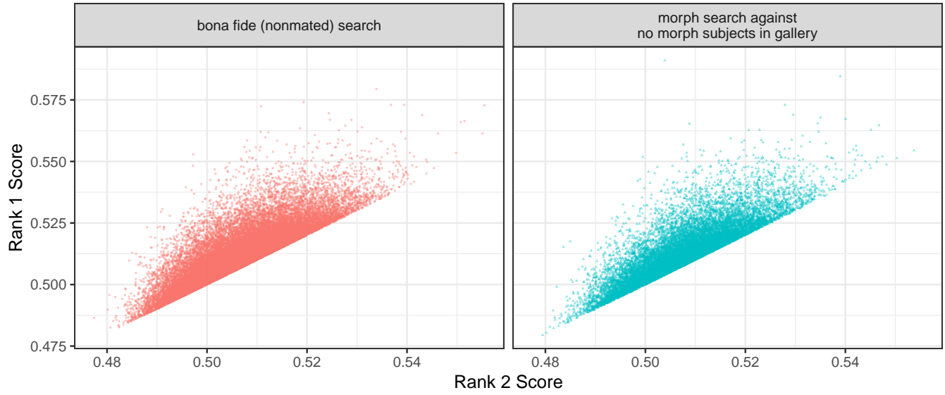
Figure 14: The position of each point in the scatter plot represents the native rank 1 and 2 similarity scores for bona fide or morph probes searched against a consolidated gallery when no prior photos of the subjects exist in the gallery. All galleries contain 1.6 million unique people.
