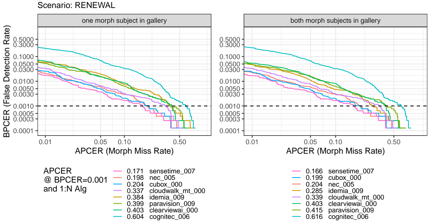
Figure 12: Accuracy of morph classifiers trained on different 1:N algorithm rank 1 + 2 scores for morphed searches (one or both subjects in gallery) and mated bona fide searches against a unconsolidated gallery.
