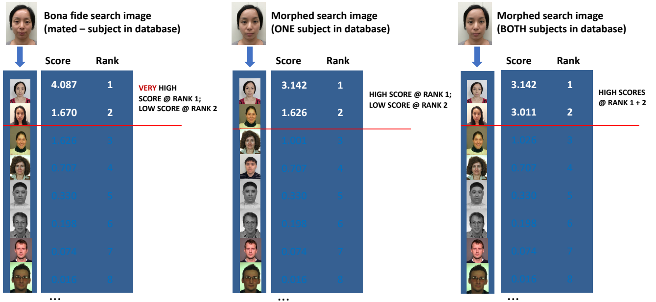
Figure 4: Notional examples of similarity scores that are returned on a candidate list for a mated search against a consolidated gallery based on 1) the type of probe (bona fide or morph) and 2) the subject(s) in the database. The images in this figure are of NIST employees + subjects from the public NIST FERET Database [14].
