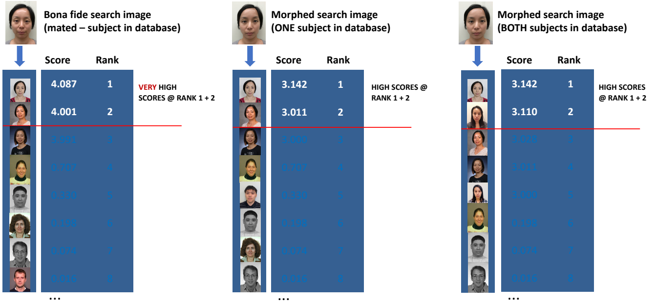
Figure 9: Notional examples of similarity scores that are returned on a candidate list for a mated search against an unconsolidated gallery where two or more images of each subject exist in the gallery. Examples show possible candidate list outcomes based on 1) the type of probe (bona fide or morph) and 2) the subject(s) in the database. The images in this figure are of NIST employees + subjects from the public NIST FERET Database [14].
