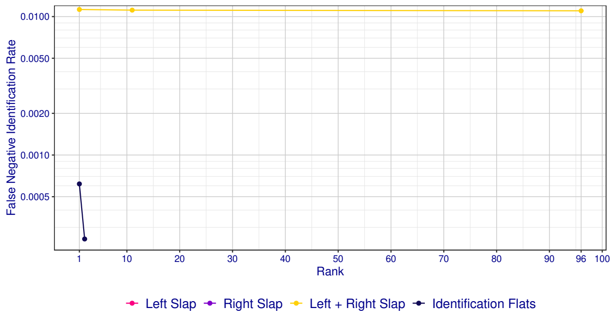
Figure 4: CMC when searching probe templates from FpVTE 2012—Class B against an enrollment database of Identification Flats.
