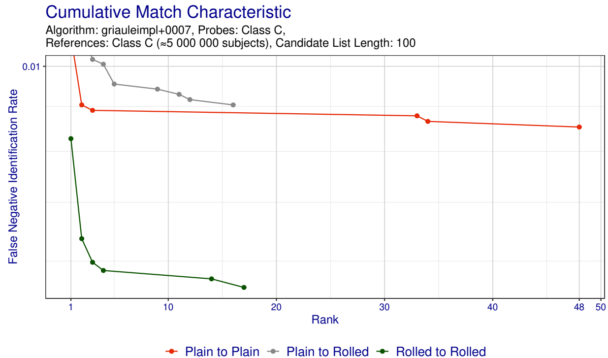
Figure 6: CMC when searching probe templates from FpVTE 2012—Class C against enrollment databases generated from reference templates from FpVTE 2012—Class C.
