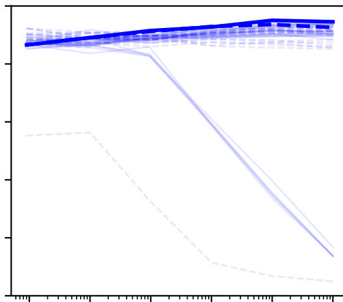
(c) petsc 3.18.5
