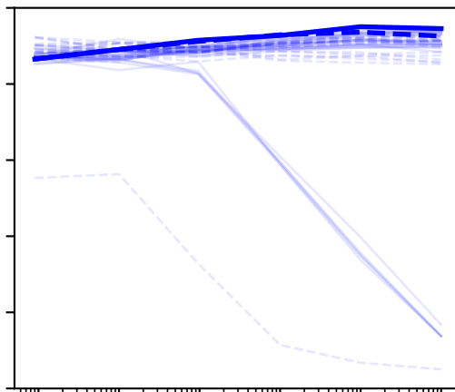
(c) petsc 3.18.5
