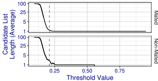
The similarity score indicated in blue is the threshold at which roc+0018 achieves 10% FPIR.
