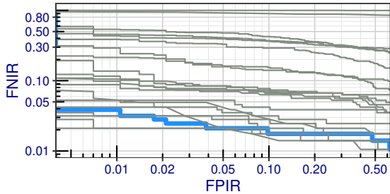
roc+0018 is highlighted in blue, alongside all other algorithms in gray (algorithms target the lower-left).
