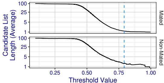
The similarity score indicated in blue is the threshold at which roc+0016 achieves 10% FPIR.
