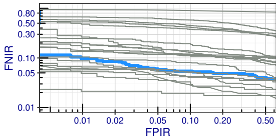
roc+0016 is highlighted in blue, alongside all other algorithms in gray (algorithms target the lower-left).
