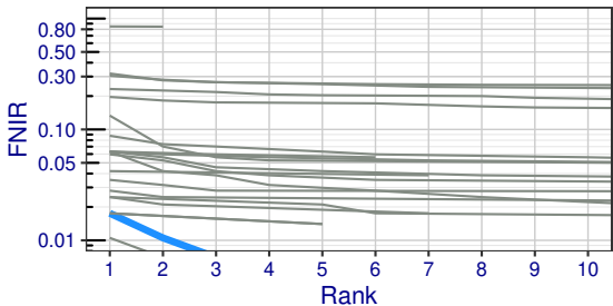
roc+0016 is highlighted in blue, alongside all other algorithms in gray (lower is better).
