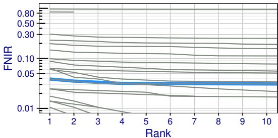
nec+0017 is highlighted in blue, alongside all other algorithms in gray (lower is better).
