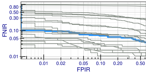
nec+0017 is highlighted in blue, alongside all other algorithms in gray (algorithms target the lower-left).
