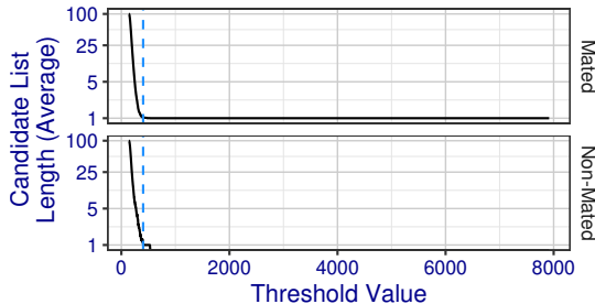
The similarity score indicated in blue is the threshold at which nec+0017 achieves 10% FPIR.
