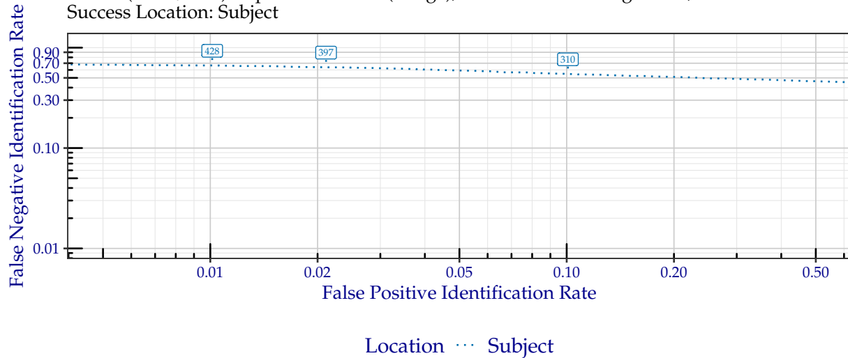
Figure 17: DET when searching IARPA N2N ( Sequestered ) probes. Annotated values indicate similarity scores from the Subject line.
