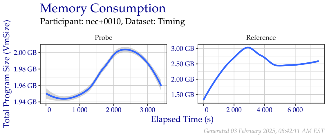
Figure 3: Amount of RAM used while creating templates in the Timing Sample dataset.
