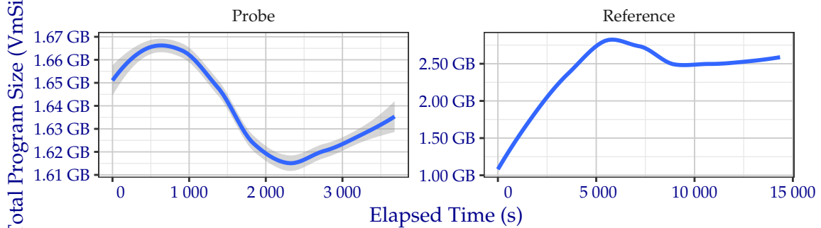
Figure 3: Amount of RAM used while creating templates in the Timing Sample dataset.
