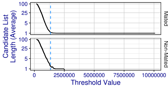
The similarity score indicated in blue is the threshold at which innovatrics+0014 achieves 10% FPIR.
