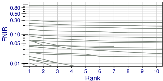
innovatrics+0014 is highlighted in blue, alongside all other algorithms in gray (lower is better).
