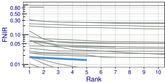
innovatrics+000E is highlighted in blue, alongside all other algorithms in gray (lower is better).
