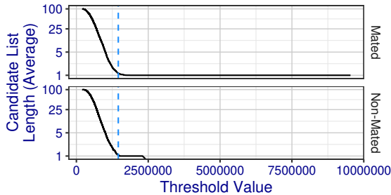
The similarity score indicated in blue is the threshold at which innovatrics+000E achieves 10% FPIR.
