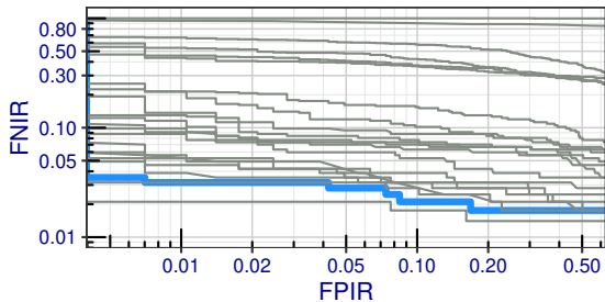
innovatrics+000E is highlighted in blue, alongside all other algorithms in gray (algorithms target the lower-left).
