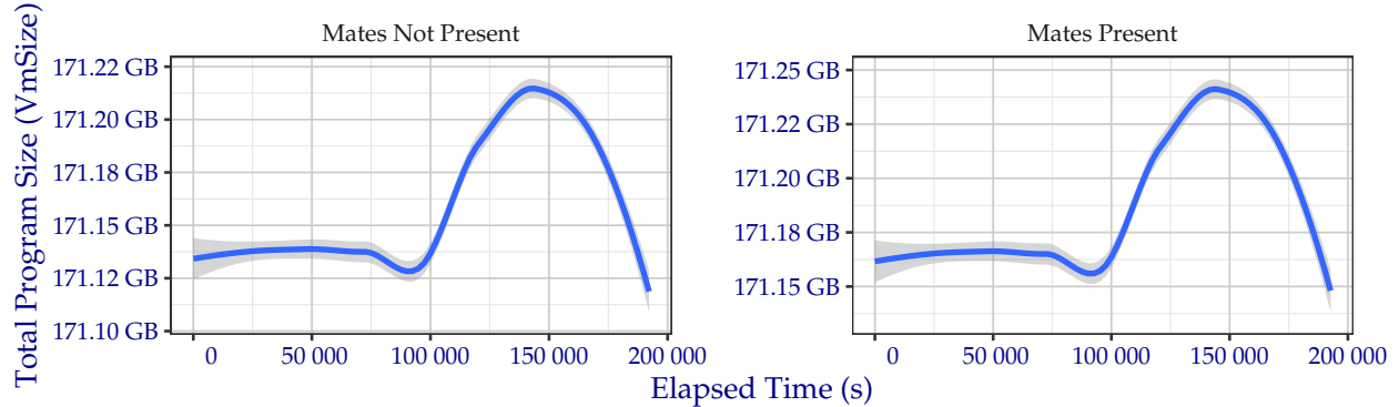
Figure 5: Amount of RAM used while searching templates in the Timing Sample dataset.
