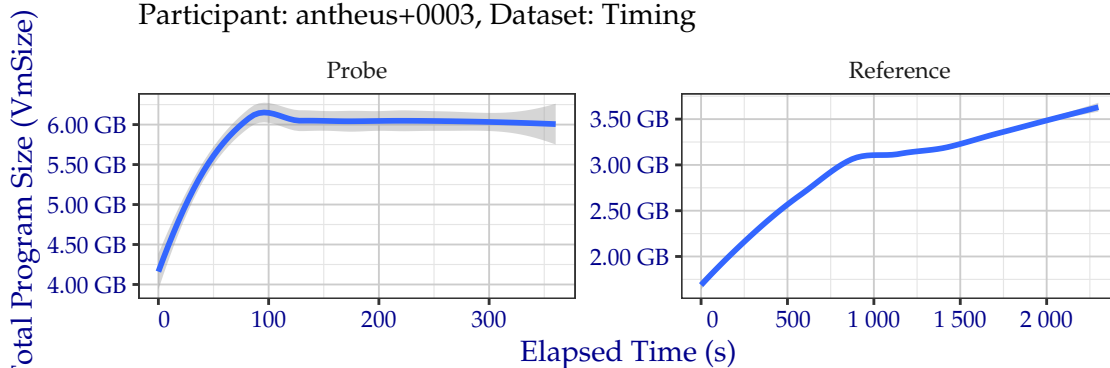
Figure 3: Amount of RAM used while creating templates in the Timing Sample dataset.
