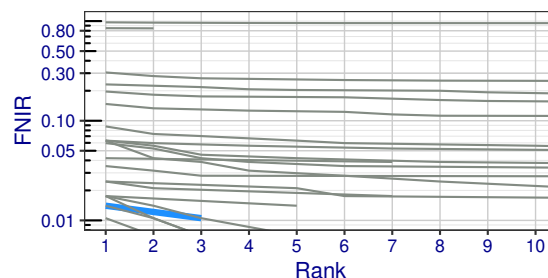
Neurotechnology+0127 is highlighted in blue, alongside all other algorithms in gray (lower is better).
