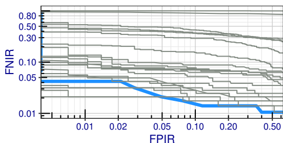
Neurotechnology+0127 is highlighted in blue, alongside all other algorithms in gray (algorithms target the lower-left).
