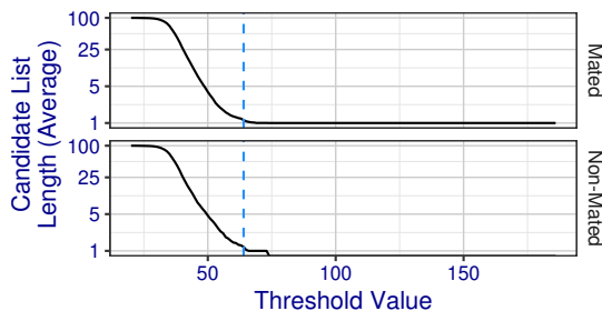
The similarity score indicated in blue is the threshold at which Neurotechnology+0127 achieves 10% FPIR.
