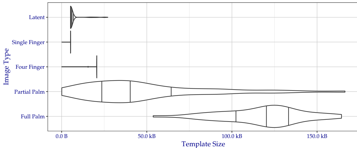
Figure 1: Violin plot of template file sizes as seen on the Timing Sample dataset. Vertical lines from left to right indicate the 25%, 50%, and 75% quantiles respectively.
